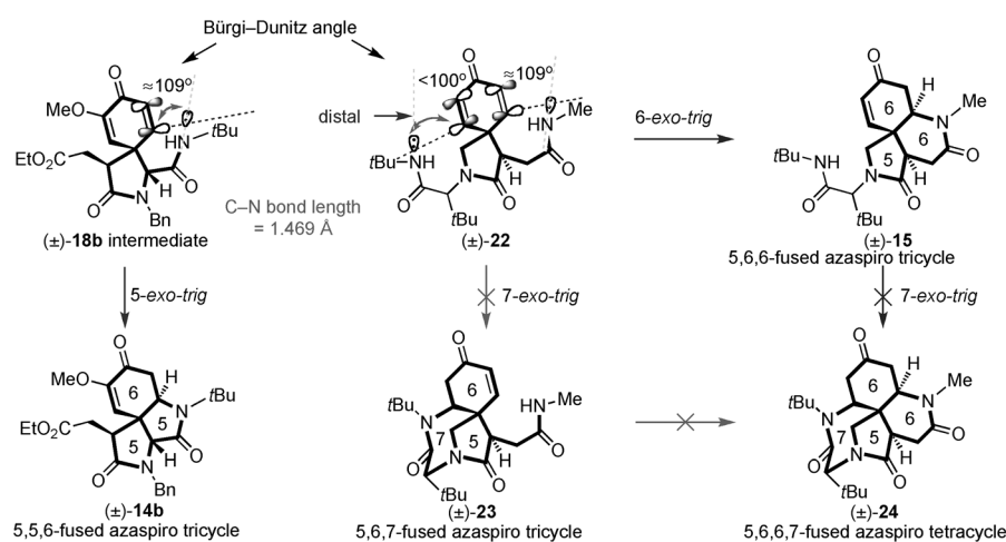
Scheme 5. Bürgi–Dunitz trajectory and proximity effect. [23a]
