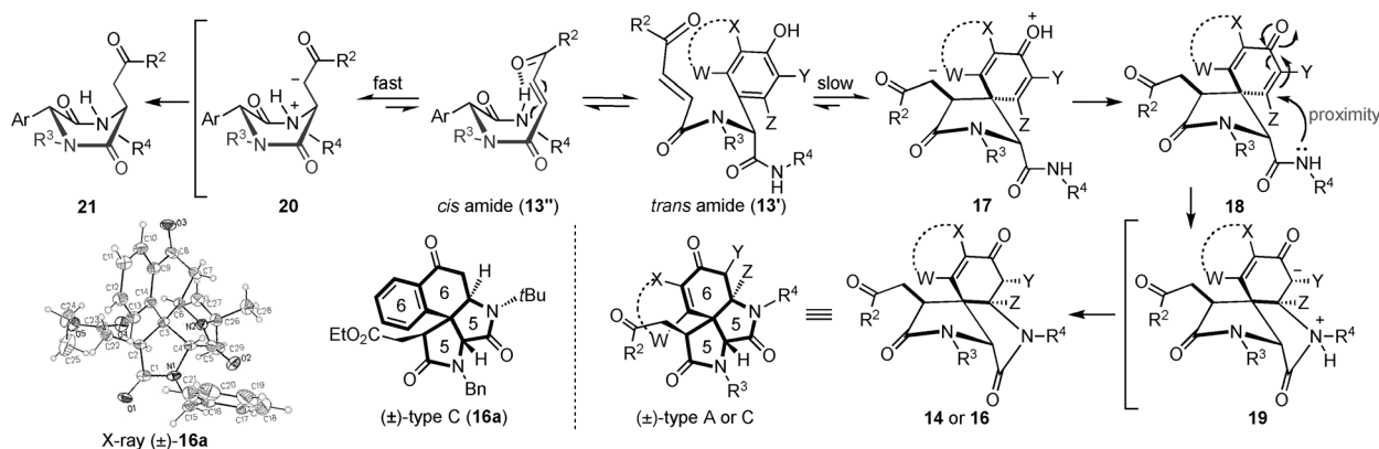
Scheme 4. Proposed mechanism for the cascade UMAM reaction.
