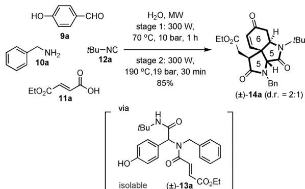
Scheme 3. Formation of 5,5,6-fused azaspiro tricycle 14a .
