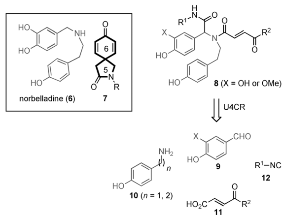
Scheme 2. Similarity between norbelladine ( 6 ) and compound 8 .
