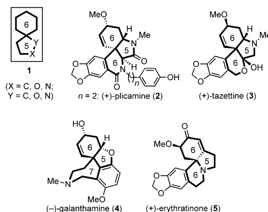
Scheme 1. Bioactive fused azaspiro polycyclic alkaloids ( 2–5 ).
